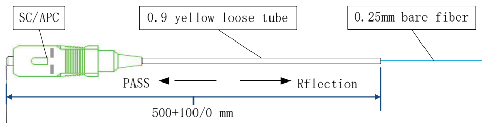
Fig : Pigtail (white) with SC/APC connector and embedded FBG
